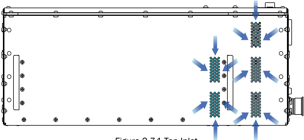
Figure 2.7.1 Top Inlet
