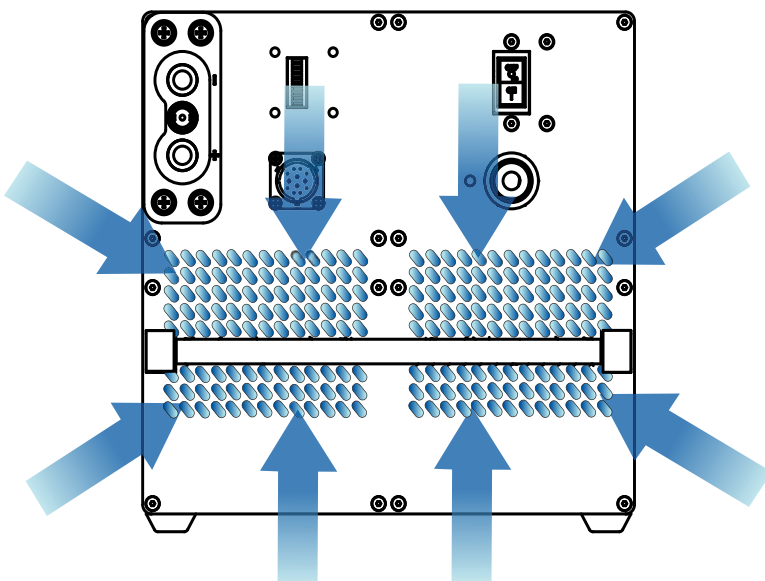
Figure 2.7.3: Front Inlet
