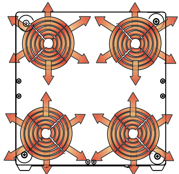
Figure 2.7.4: Rear Outlet
