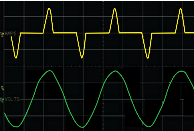
Figure 2.8.1 - Non-PFC Power Supply
